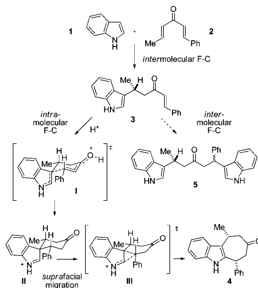
Scheme 3. Partial Mechanistic Rationale for the Formation of Fused Tricyclic Indoles from Divinyl Ketones
