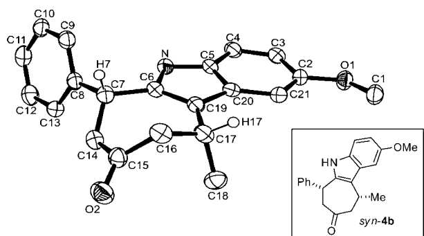
Figure 1. ORTEP plot of syn - 4b (ellipsoids at 30% probability).
