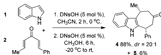
Scheme 2. Improved Two-Step, Solvent Substitution Protocol
